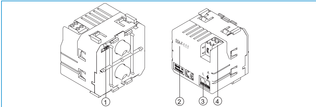
Fig. 2: Device overview of sensor/switch actuator 1/1gang and 2/1gang
